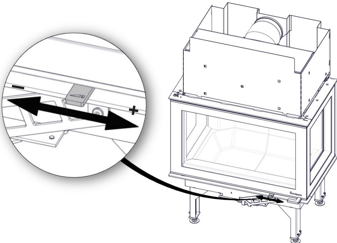
FIG 8 Operational control
