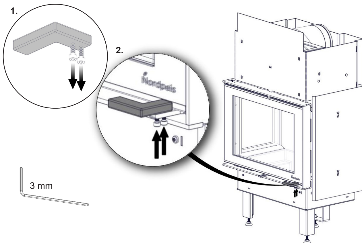
FIG 9 Operational handle assembling
