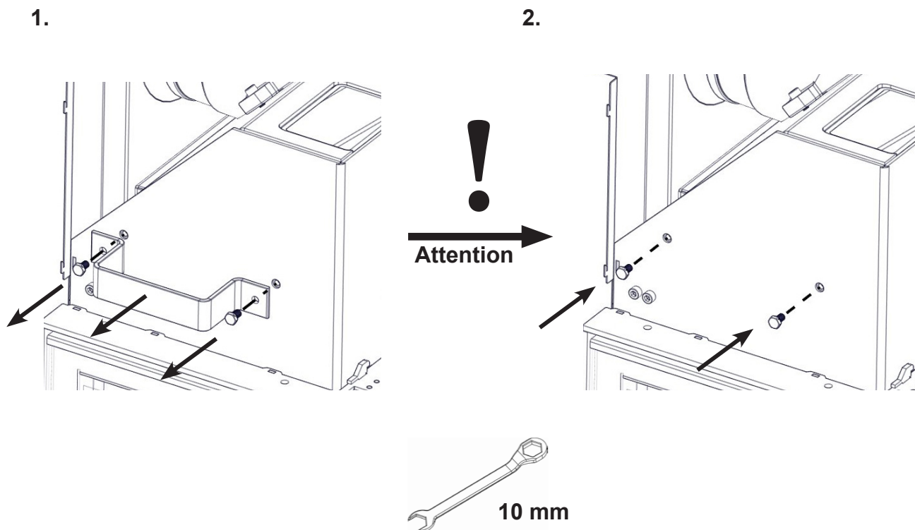
FIG 7 Front radiation shield - assembling
