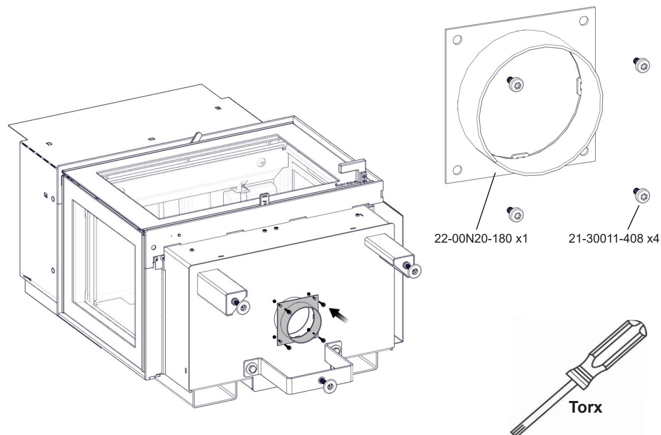
FIG 4 Air inlet pipe assembling
