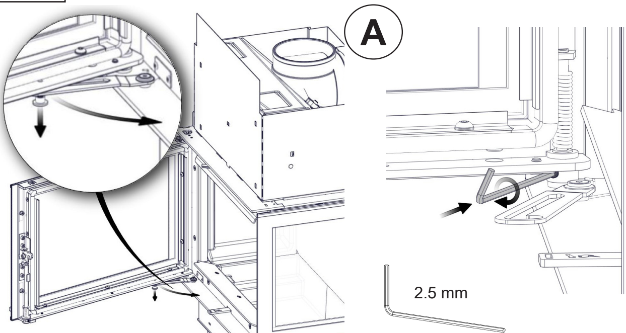
FIG 16 Self-closing door deactivation
