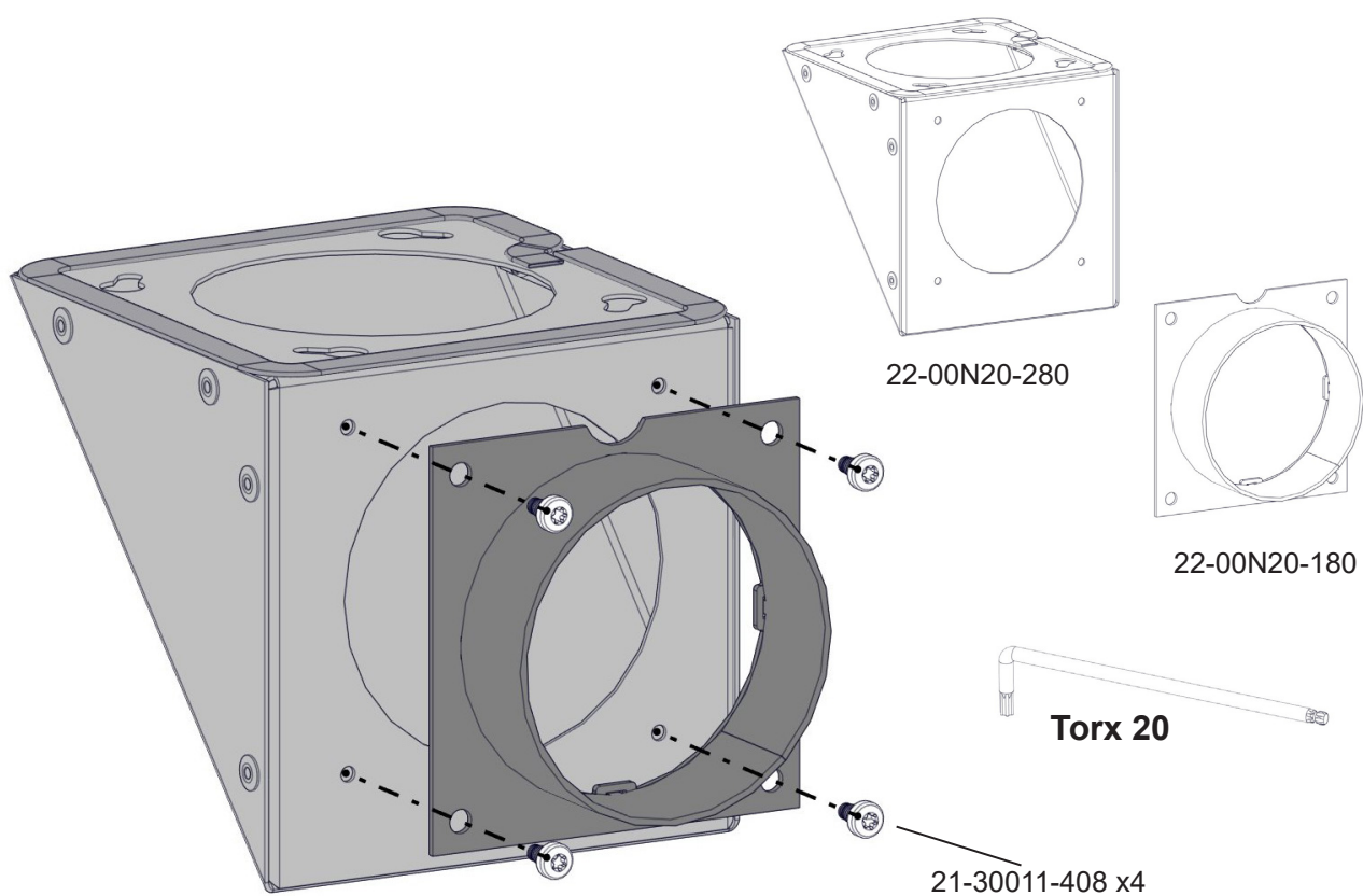
FIG 4 a Air inlet adapter 90° assembling - optional
