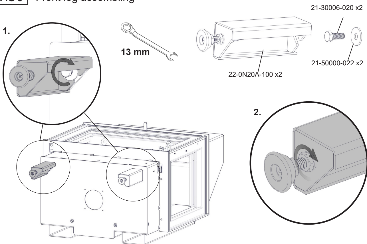
FIG 3 Front leg assembling
