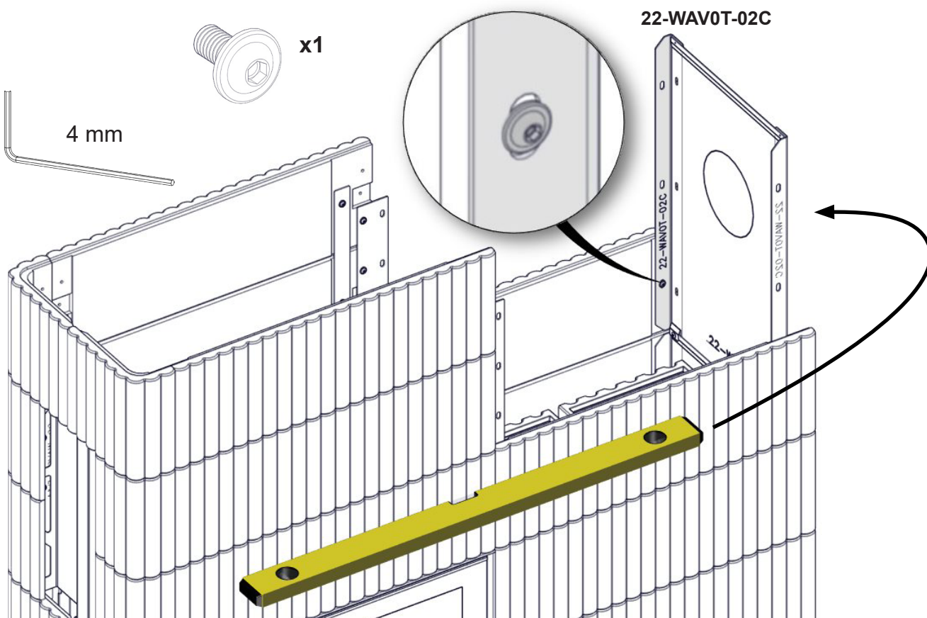
FIG 32 b Wave T 3+3 Wide with Powerbox L
