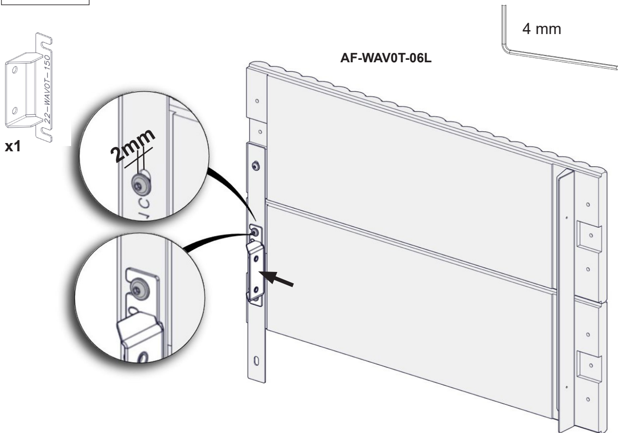
FIG 19 Wave T 3+3 Wide with Powerbox L
