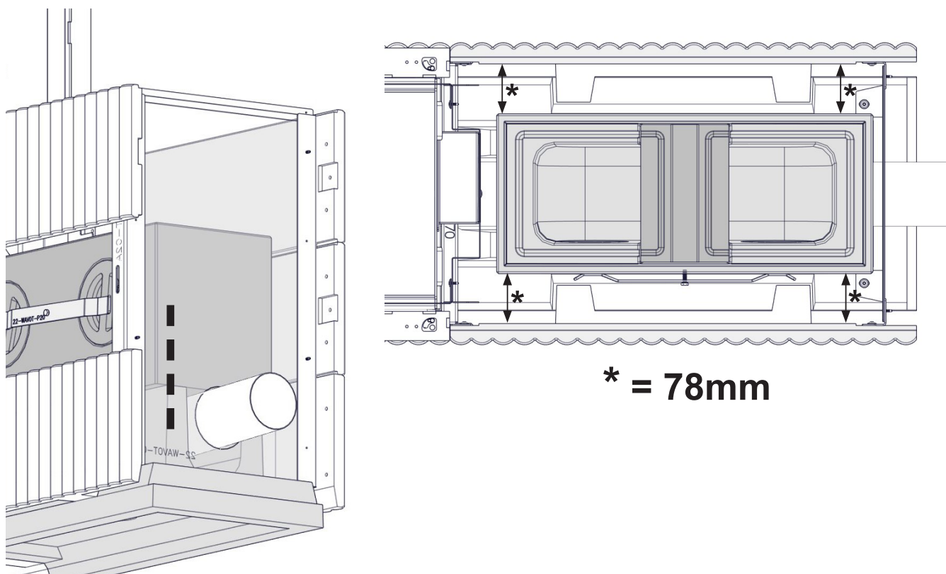
FIG 15 b Wave T 3+3 Wide with Powerbox L
