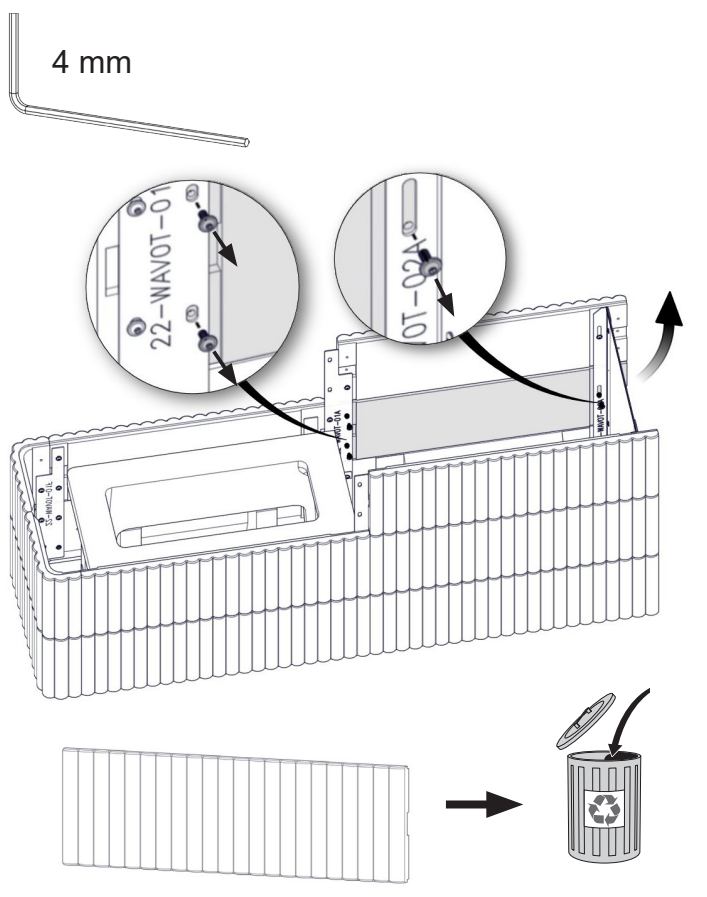
FIG 12 Wave T 3+3 Wide with Powerbox L
