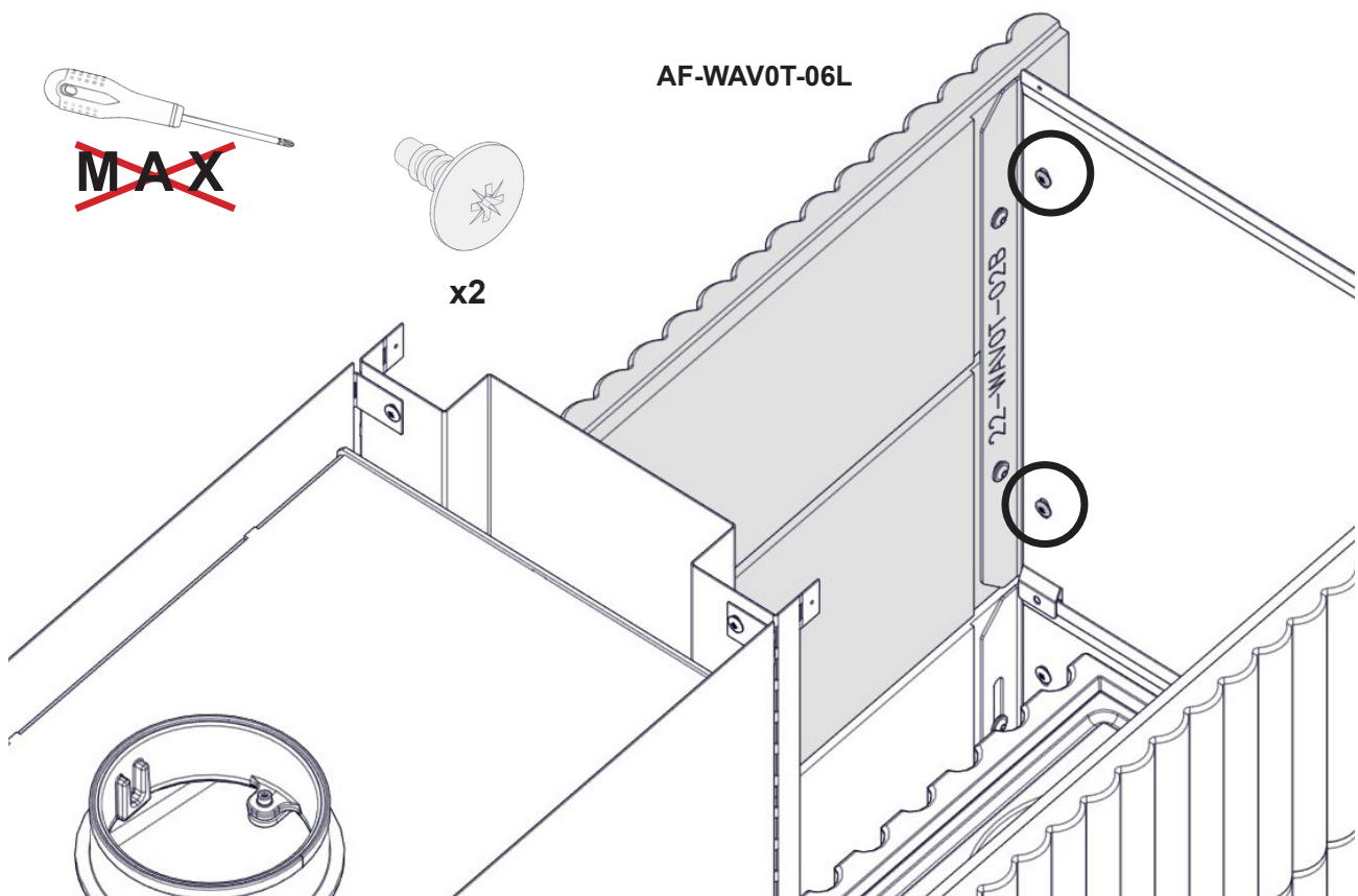
FIG 19 a Wave T 3+3 Wide with Powerbox L
