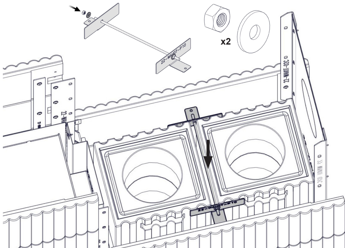
FIG 36 a Wave T 3+3 Wide with Powerbox L
