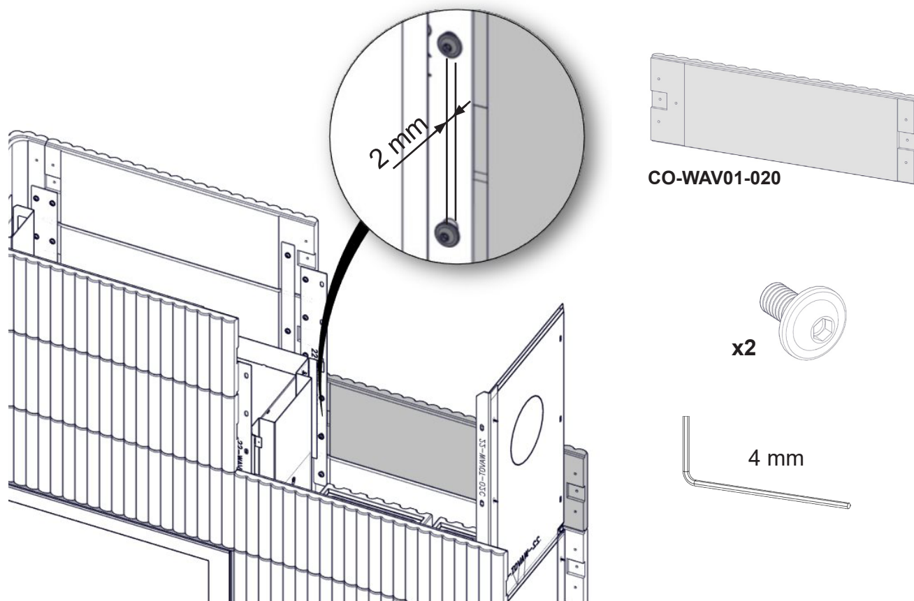
FIG 32 Wave T 3+3 Wide with Powerbox L
