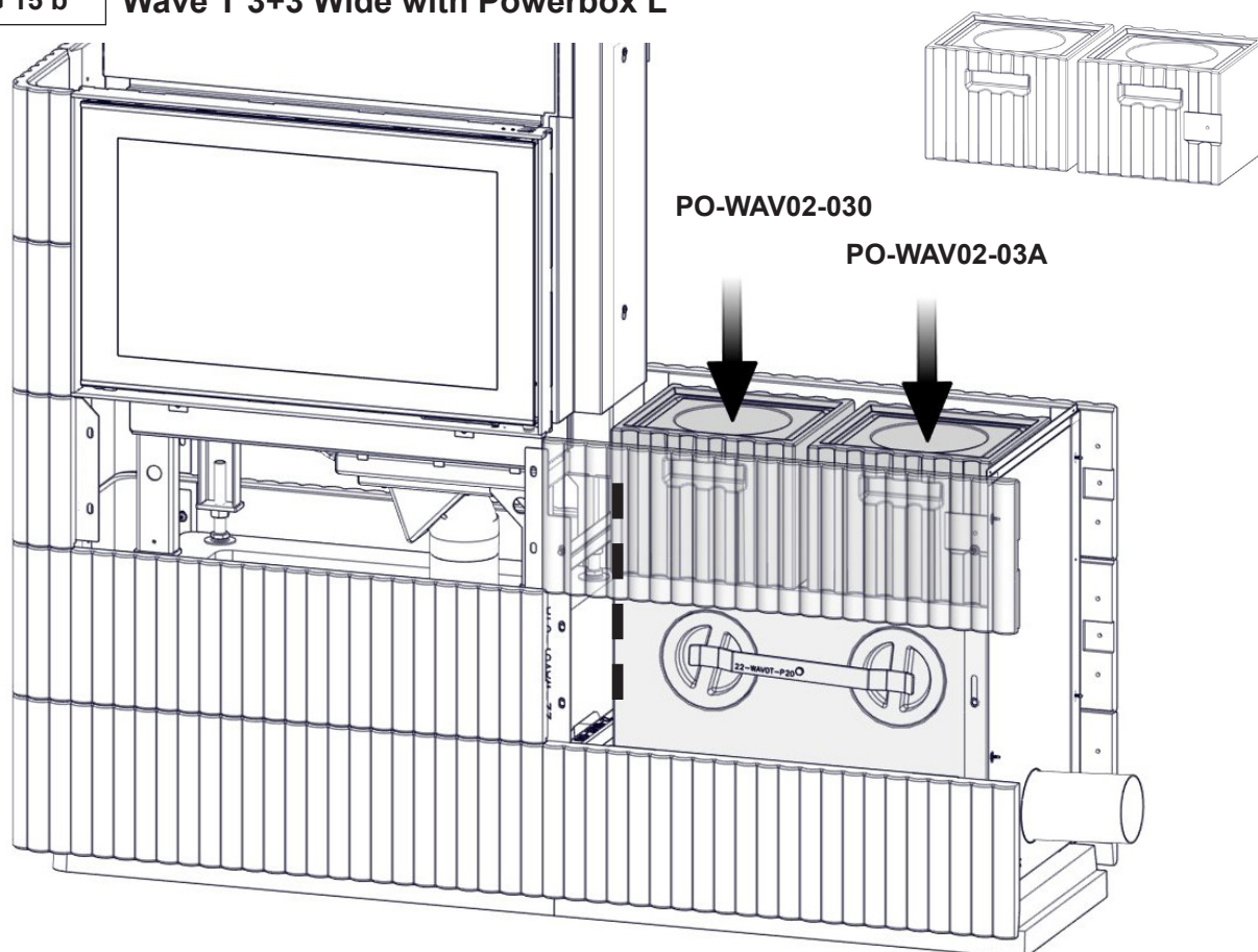
FIG 15 b Wave T 3+3 Wide with Powerbox L
