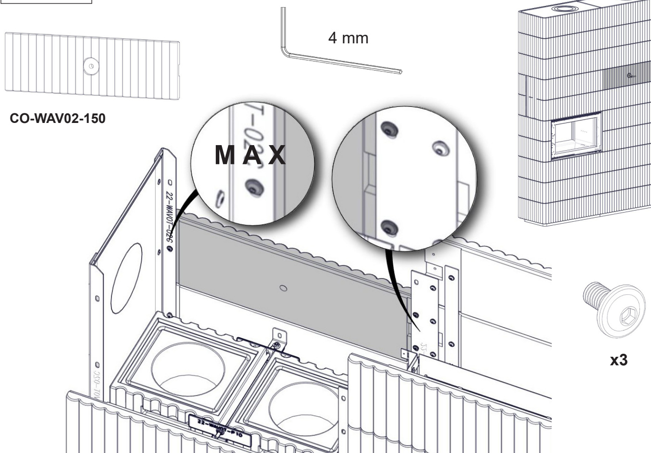
Wave T 3+3 Wide with Powerbox L
