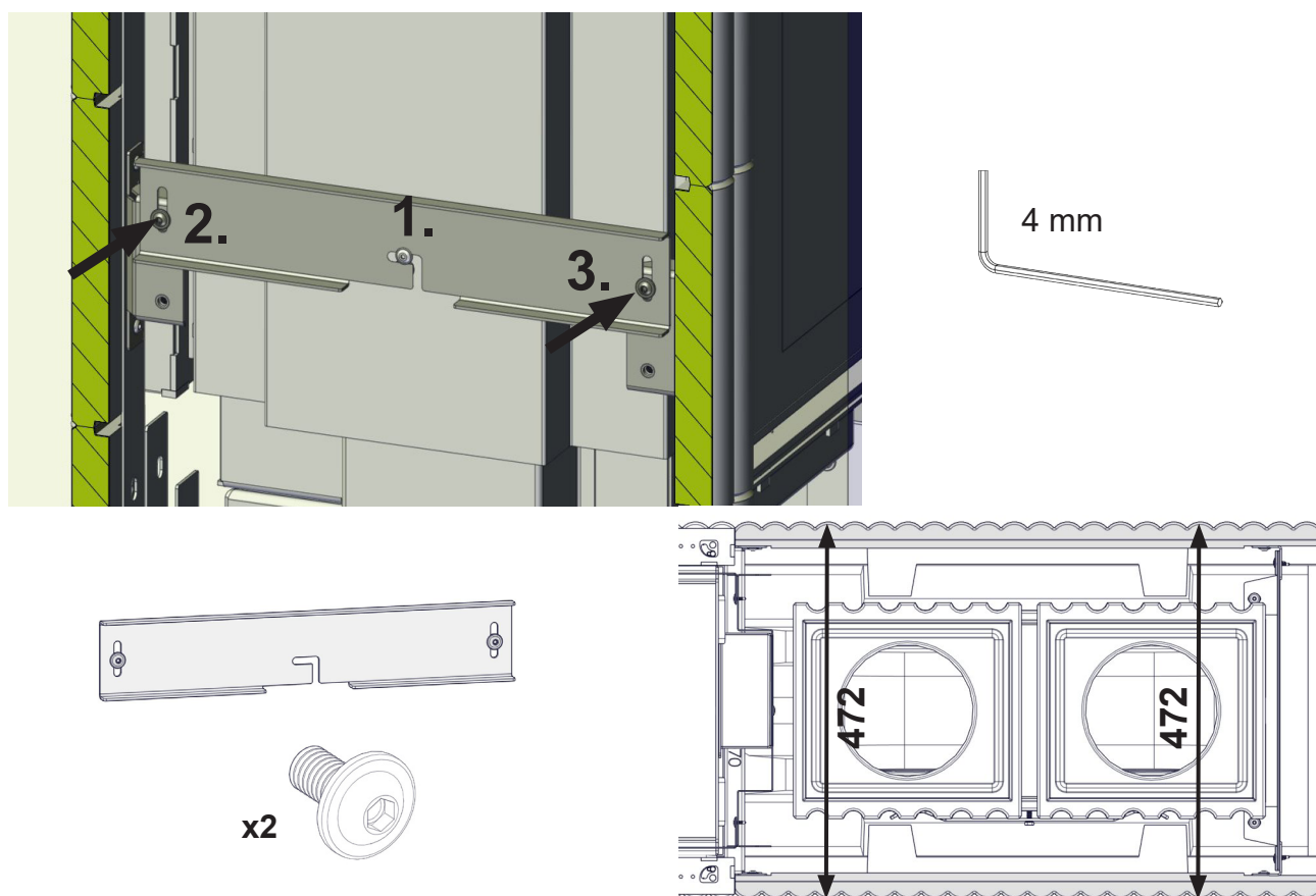
Wave T 3+3 Wide with Powerbox L
