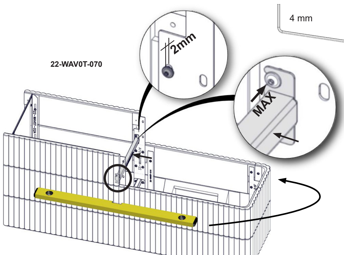
FIG 10 Wave T 3+3 Wide with Powerbox L
