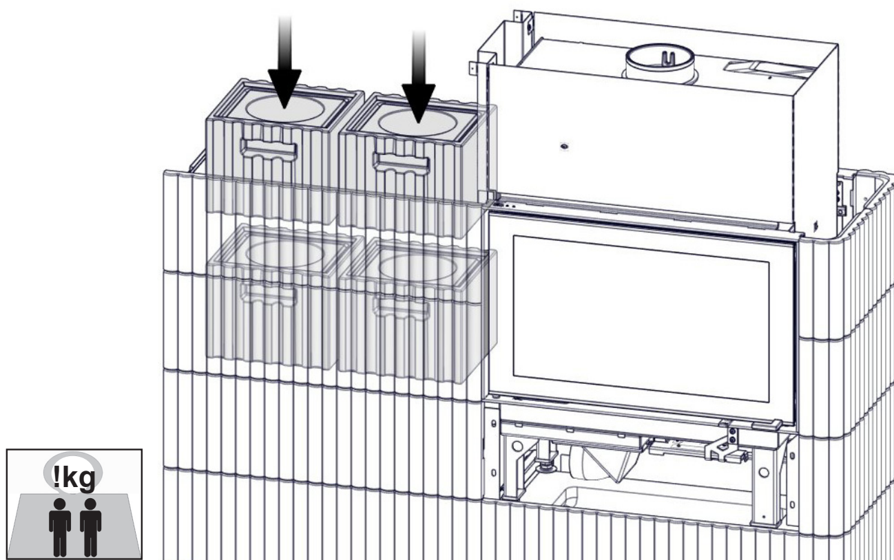
Wave T 3+3 Wide with Powerbox L
