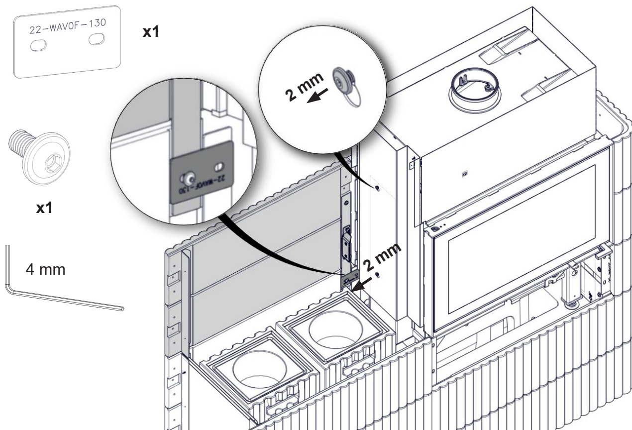
FIG 18 Wave T 3+3 Wide with Powerbox L
