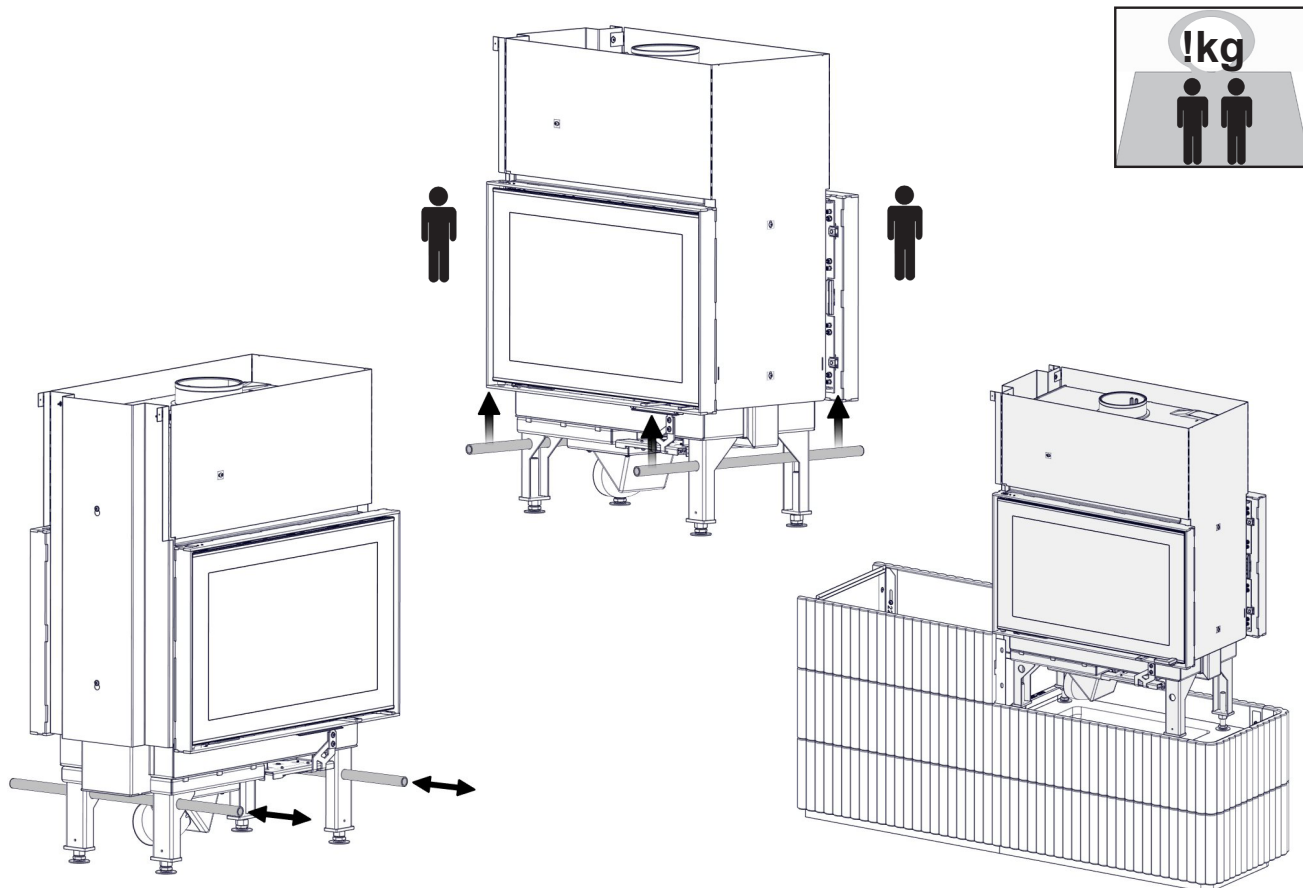
FIG 12 a Wave T 3+3 Wide with Powerbox L
