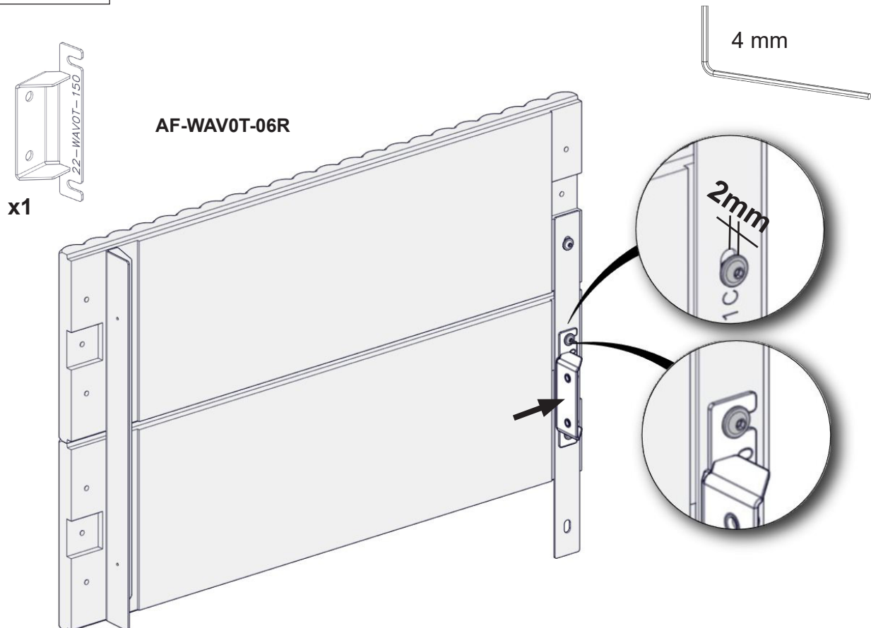
Wave T 3+3 Wide with Powerbox L
