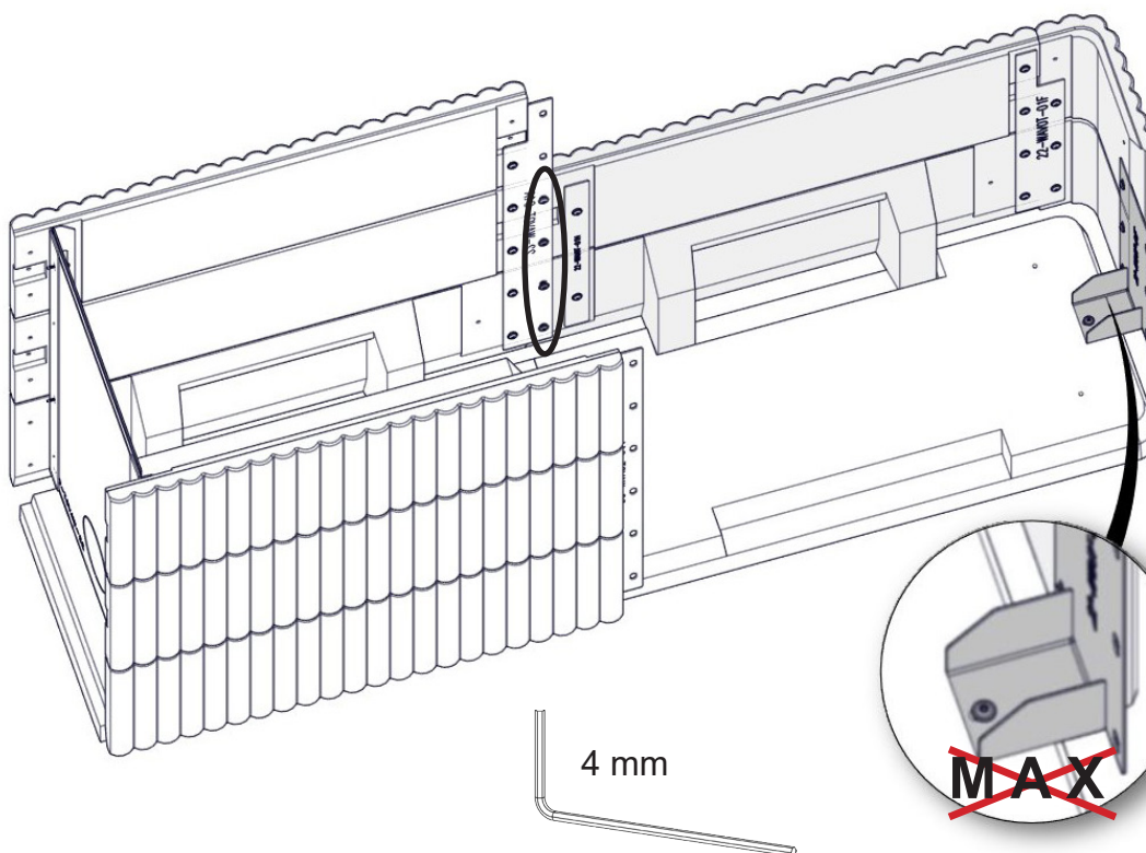
Wave T 3+3 Wide with Powerbox L
