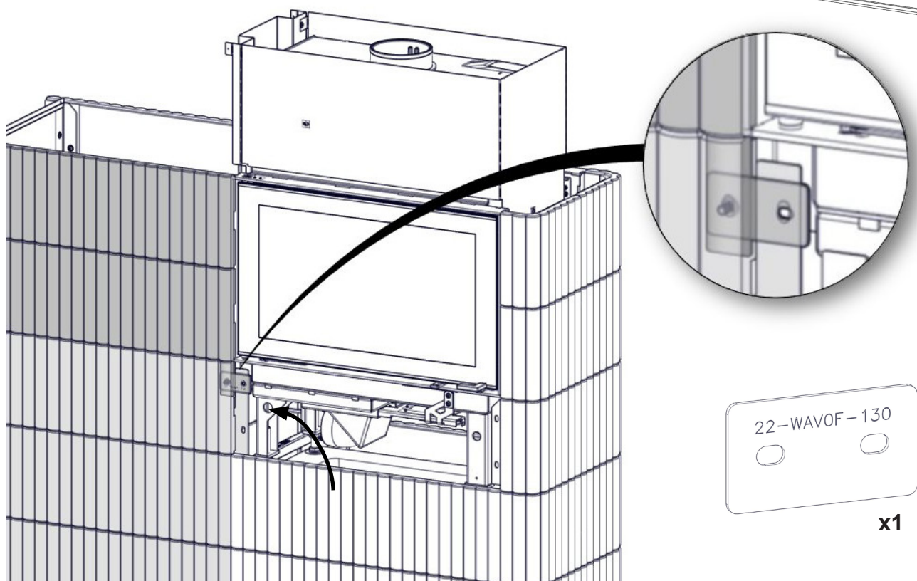
Wave T 3+3 Wide with Powerbox L
