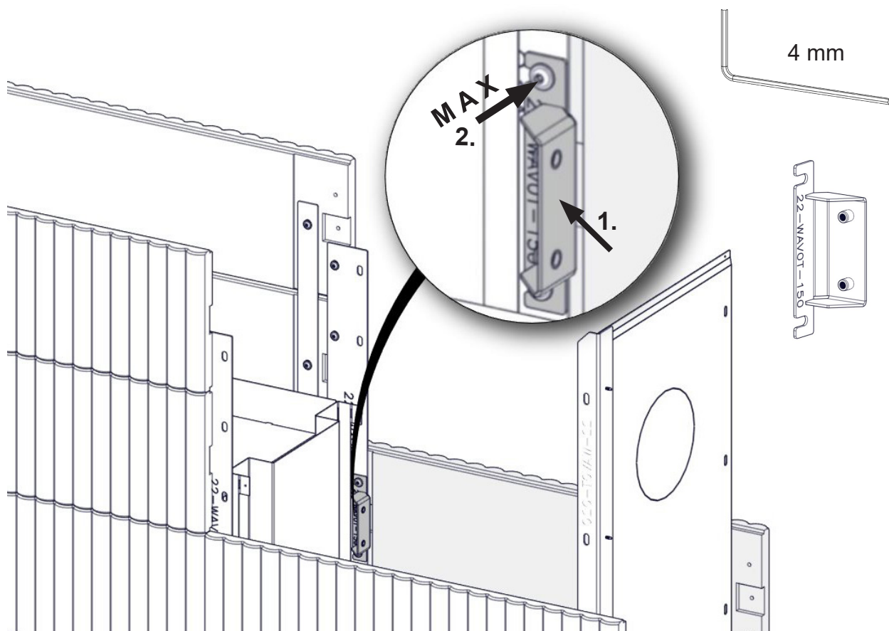
FIG 32 b Wave T 3+3 Wide with Powerbox L
