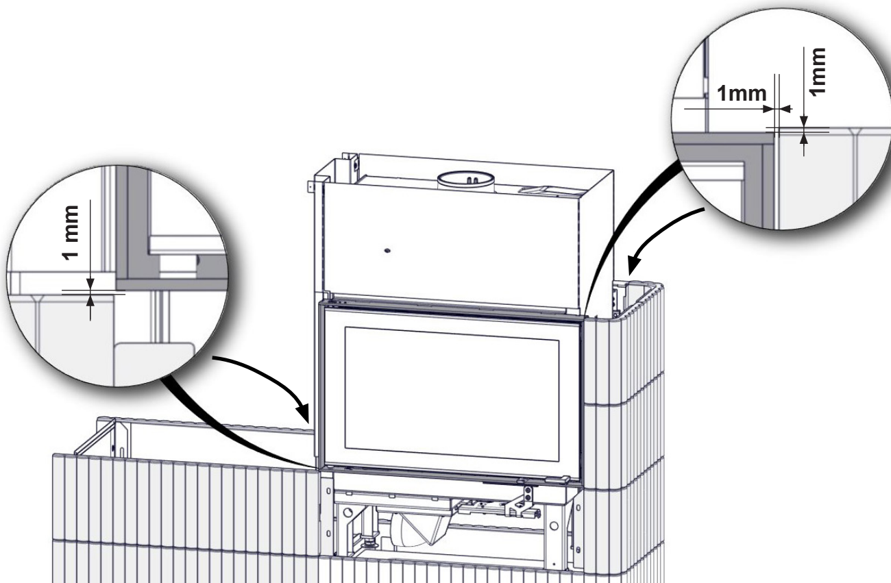
FIG 14 Wave T 3+3 Wide with Powerbox L
