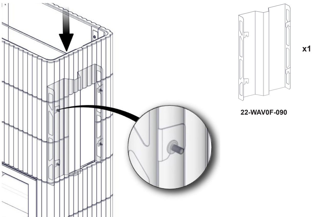
FIG 29 a Wave T 3+3 Wide with Powerbox L
