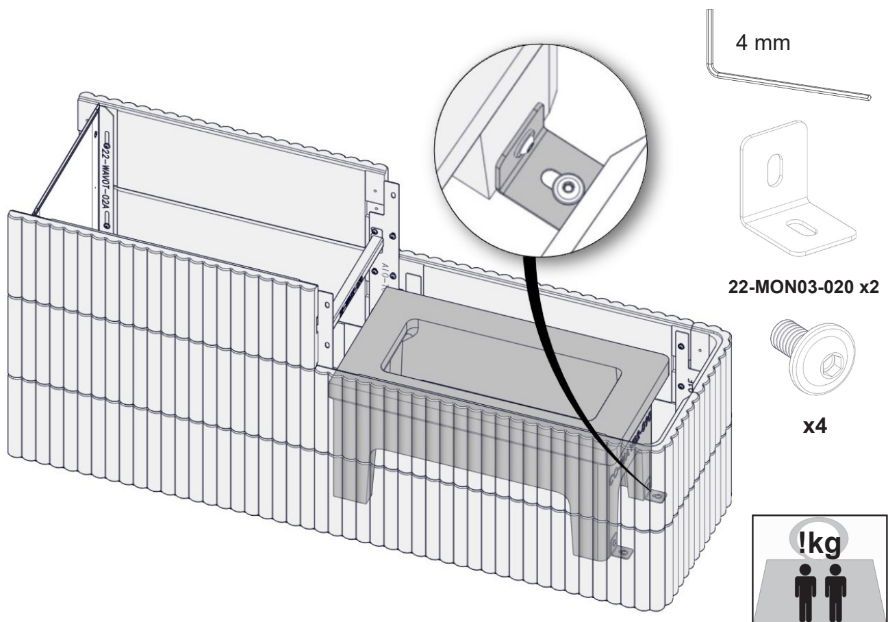
FIG 10 a Wave T 3+3 Wide with Powerbox L
