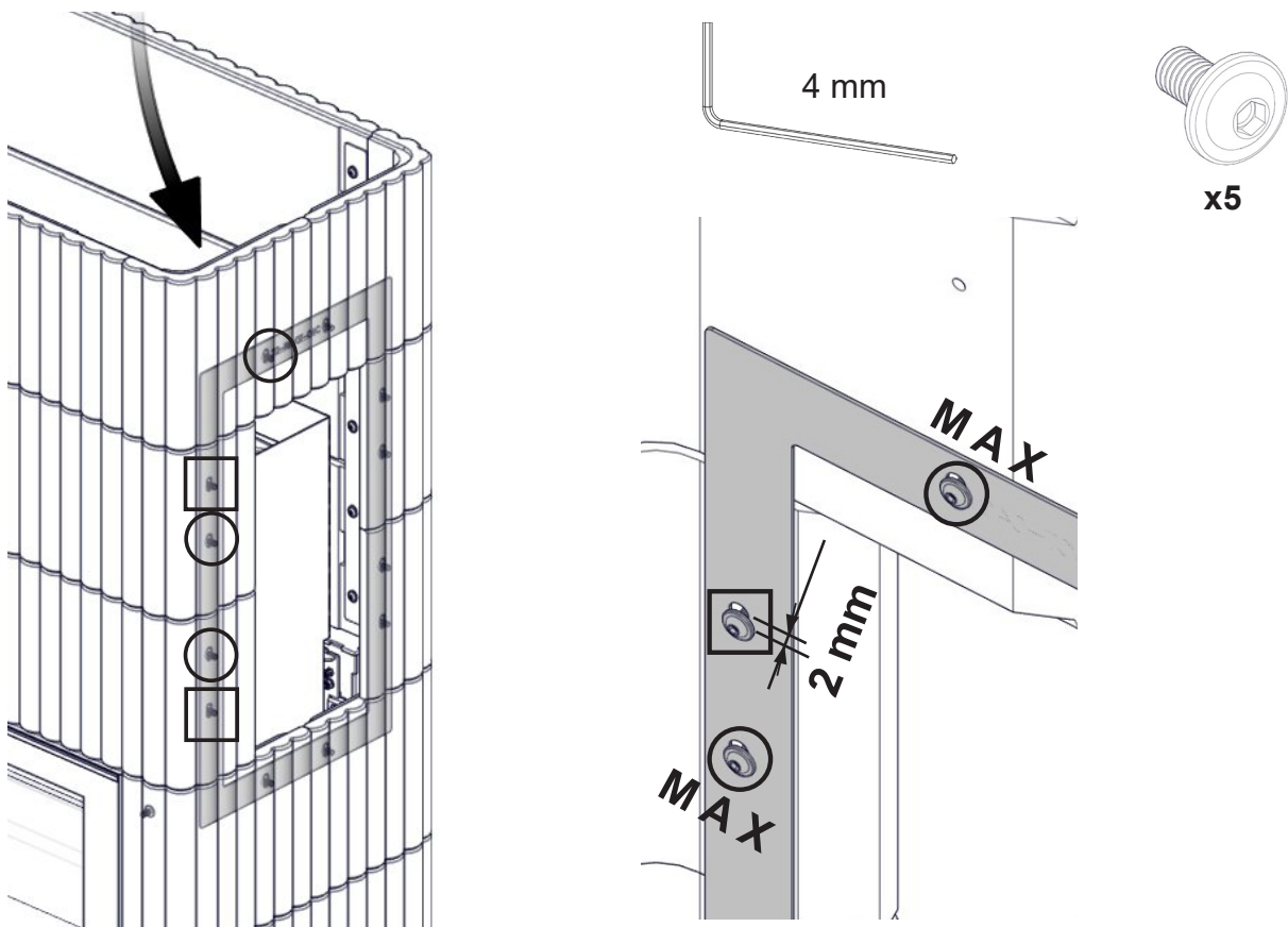
FIG 29 Wave T 3+3 Wide with Powerbox L
