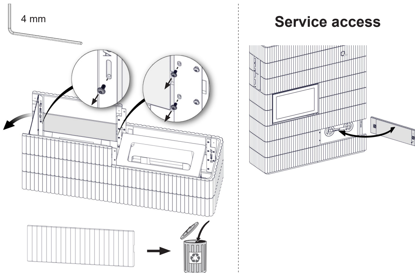
FIG 11 Wave T 3+3 Wide with Powerbox L
