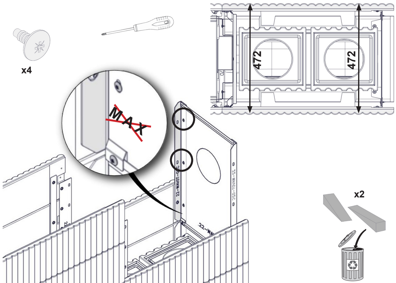
Wave T 3+3 Wide with Powerbox L
