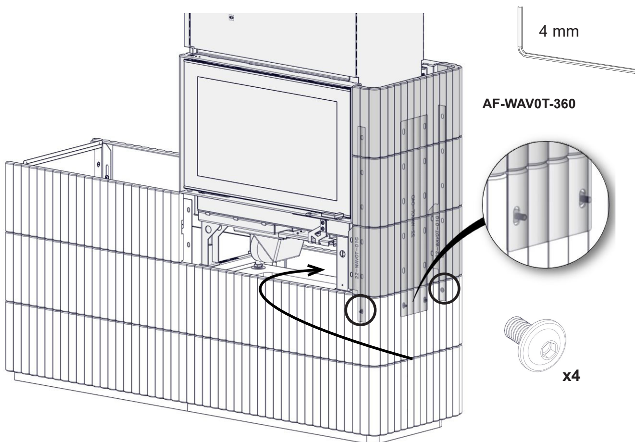
FIG 13 Wave T 3+3 Wide with Powerbox L
