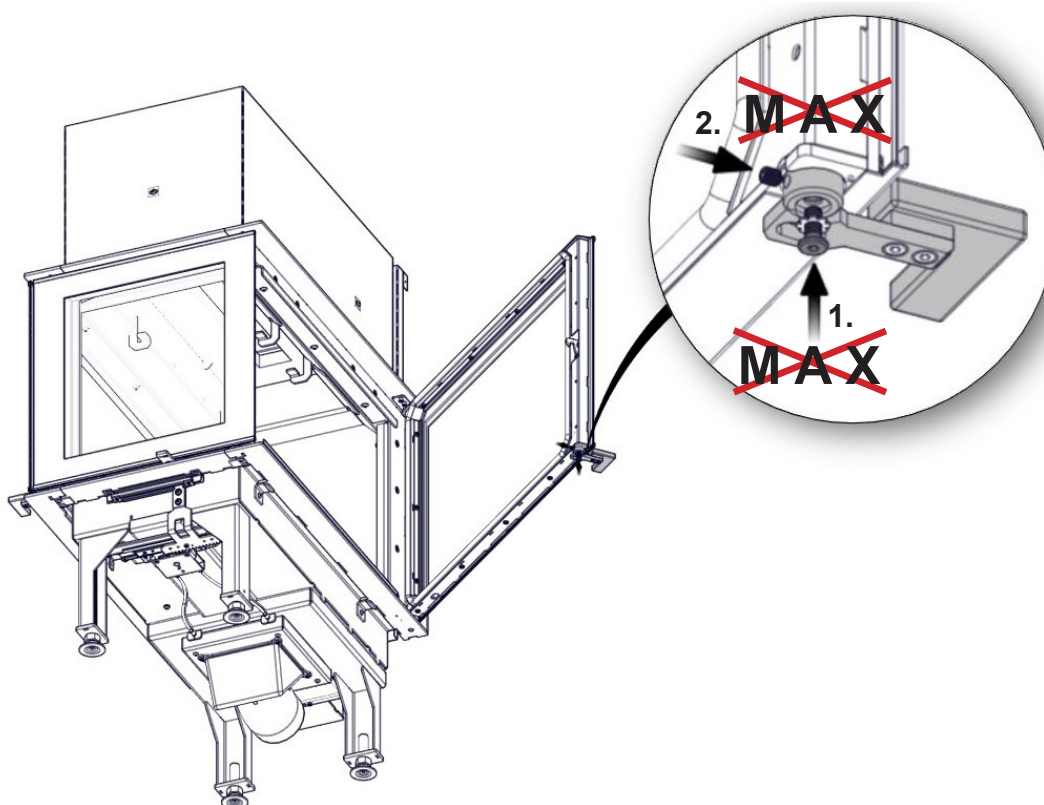
FIG 5 c Right door handle assembling
