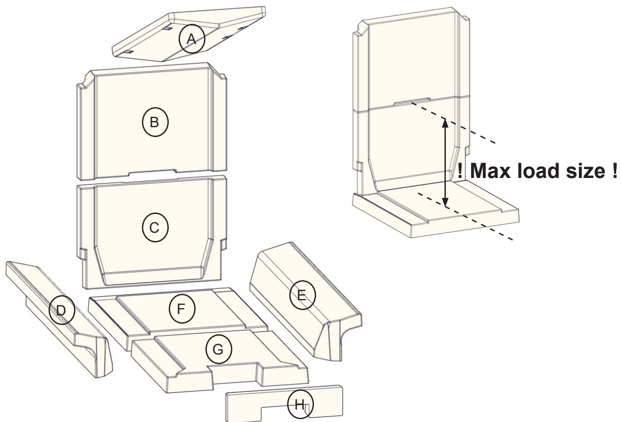
FIG 11 Thermotte assembling
