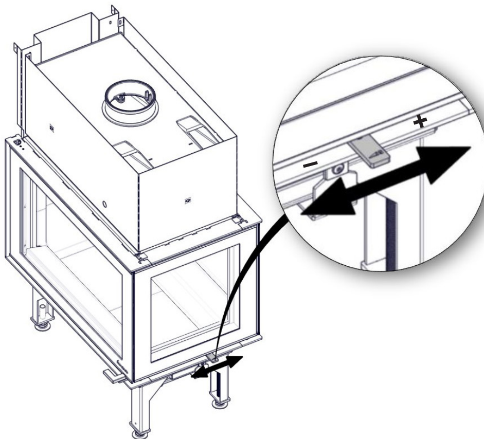
FIG 9 Smoke adapter - back chimney connection
