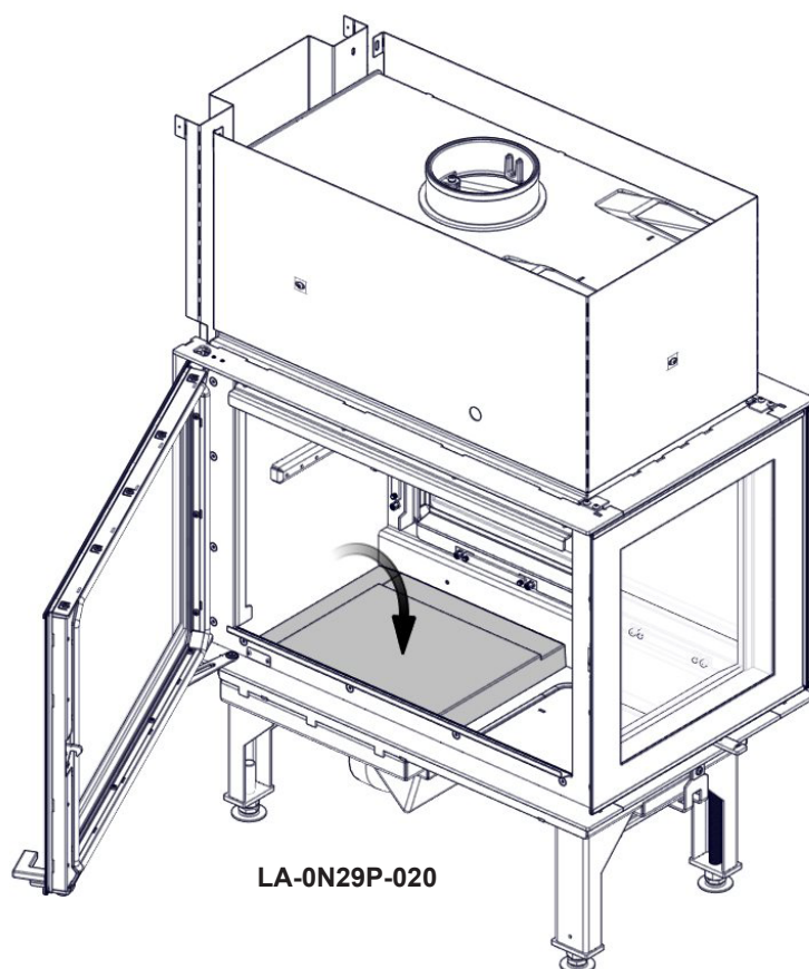
FIG 11 Thermotte assembling
