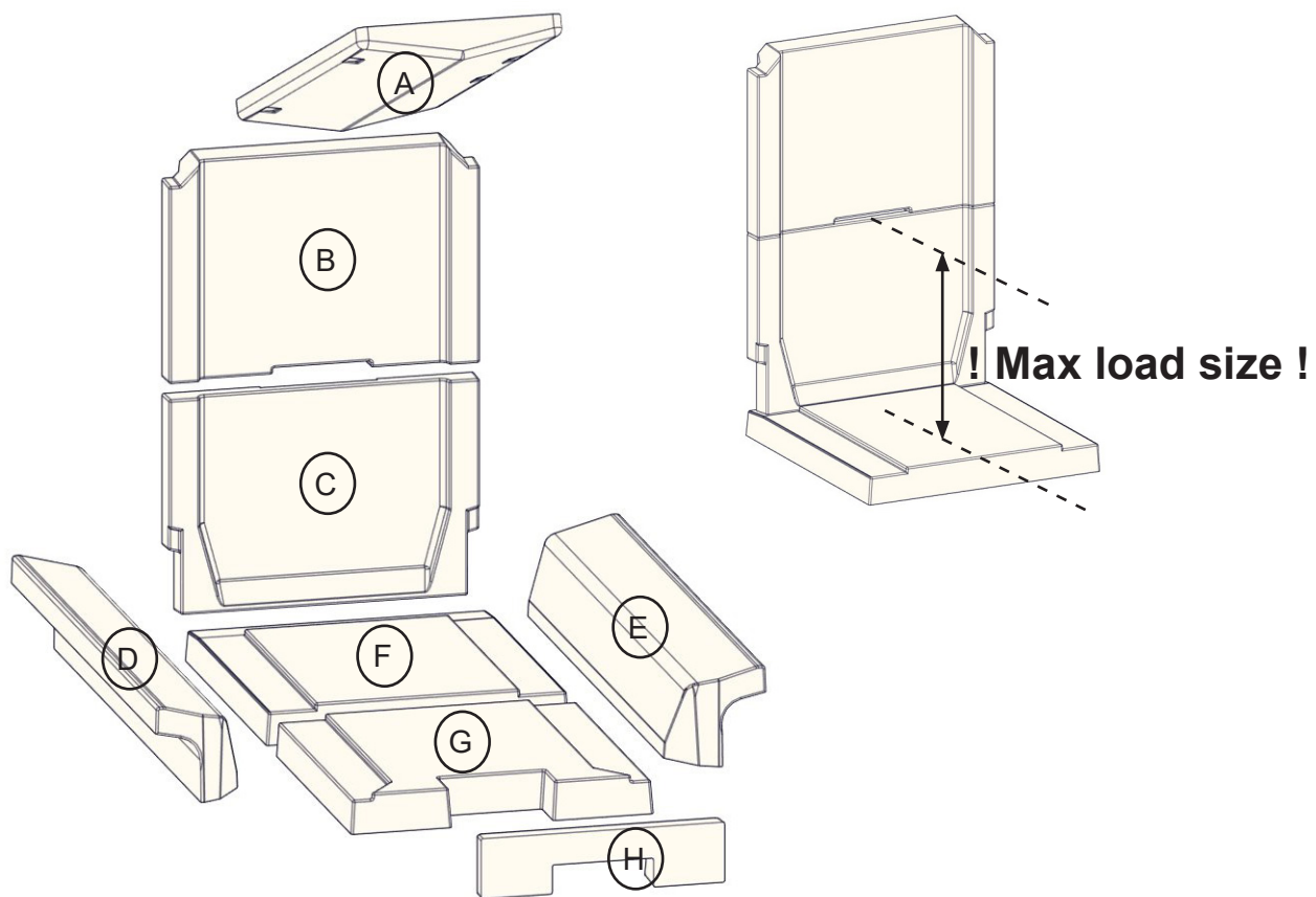
FIG 11 Thermotte
