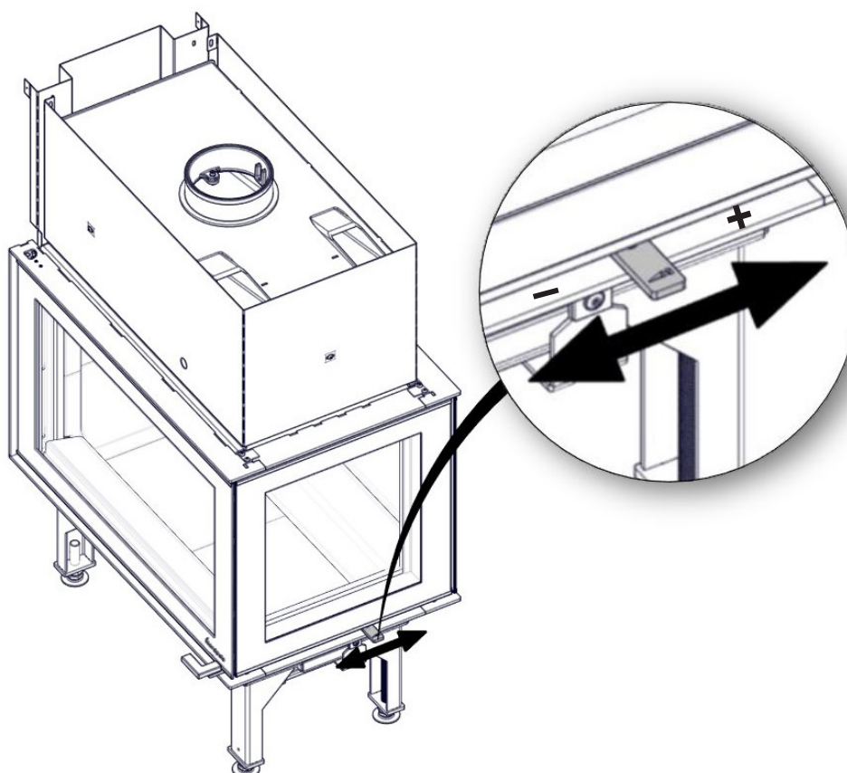
FIG 8 Operational control
