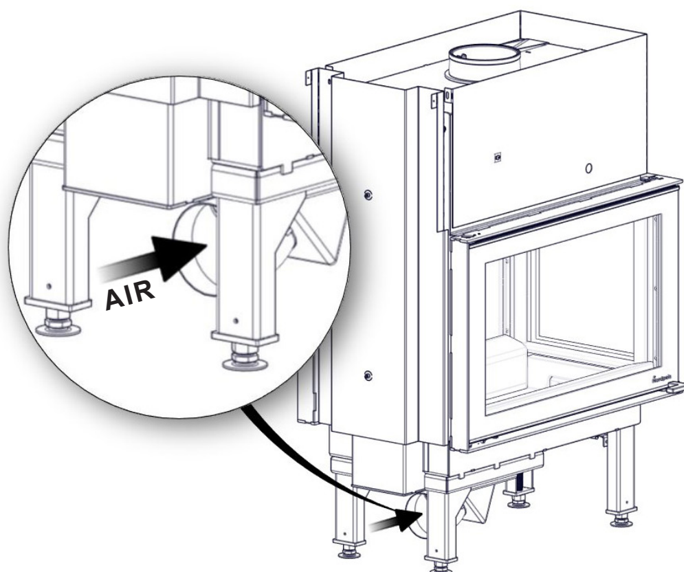
FIG 6 Air inlet
